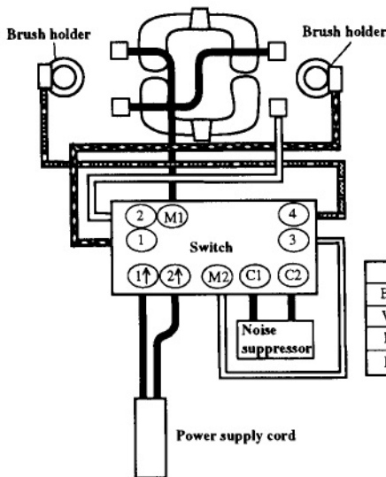
Wiring Diagram
